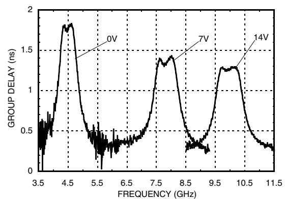
Group Delay
