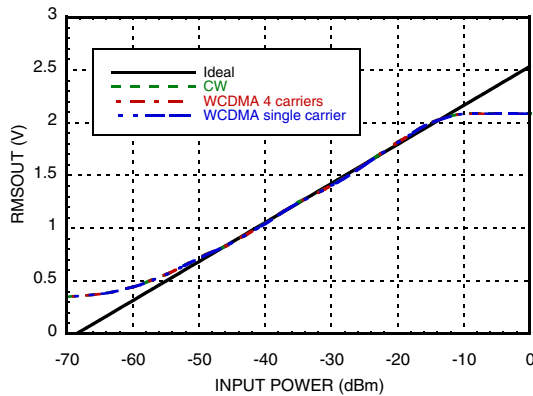
RMSOUT vs. Pin with Different Modulations @ 1900 MHz [1]
