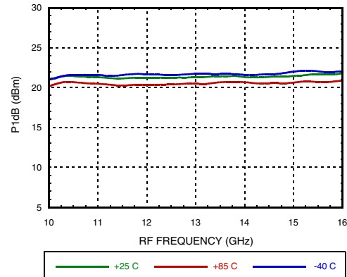
Output P1dB, USB vs. Temperature
