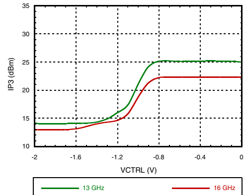
Input IP3, USB vs. Control Voltage
