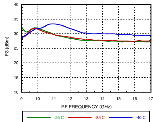
Output IP3, USB vs. Temperature
