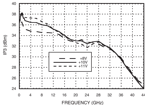
Output IP3 vs. Supply Voltage @ Pout = 14 dBm / Tone
