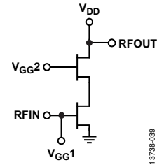
Figure 35. Fundamental Cell Schematic
