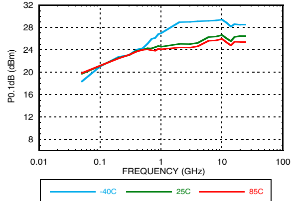
Input Power for 0.1 dB Compression
