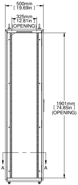
L.S. VIEW
