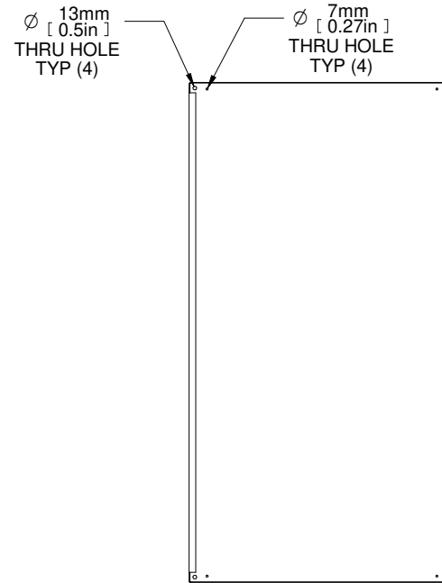
REAR VIEW
