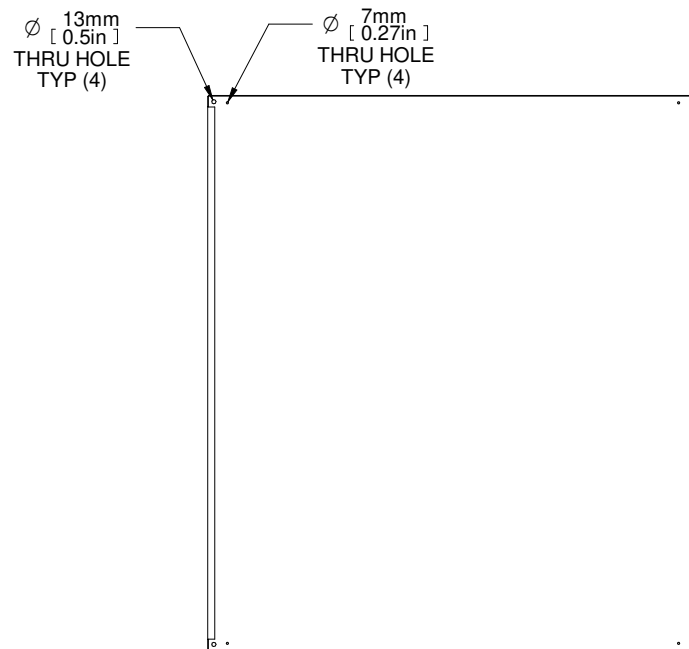
REAR VIEW
