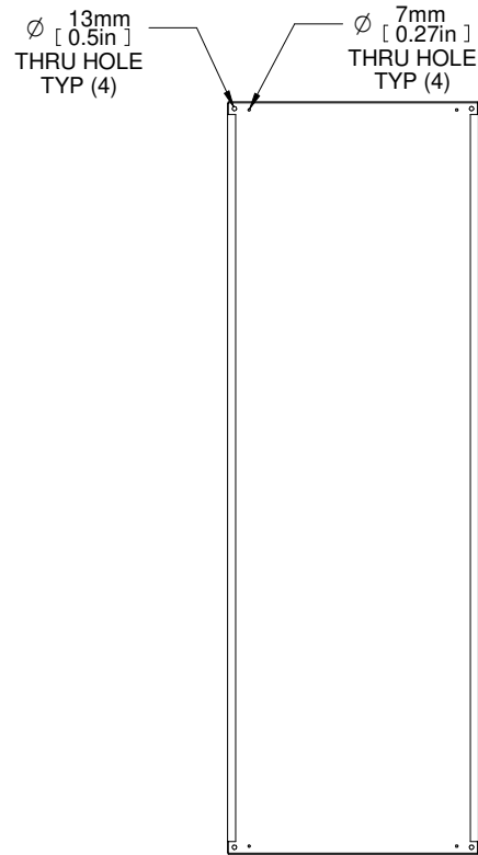
REAR VIEW
