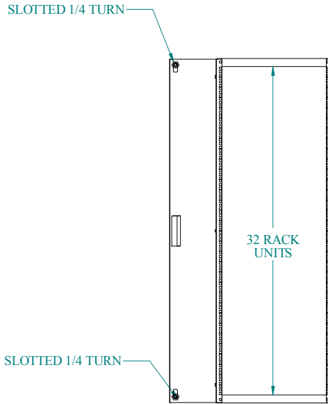
REAR VIEW
