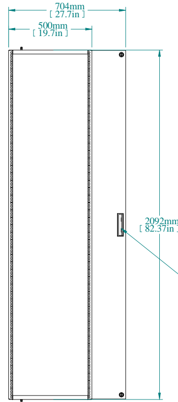
FRONT VIEW
