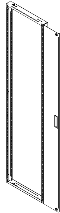
ISOMETRIC VIEW
