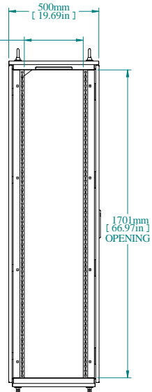
L.S. VIEW
