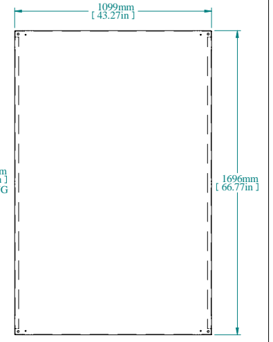
INNER PANEL
