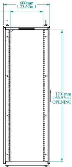
L.S. VIEW
