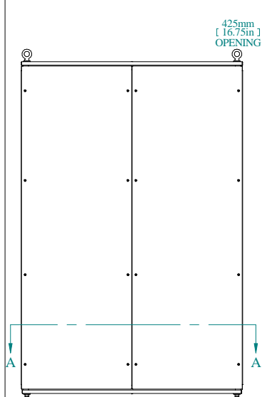
REAR VIEW
