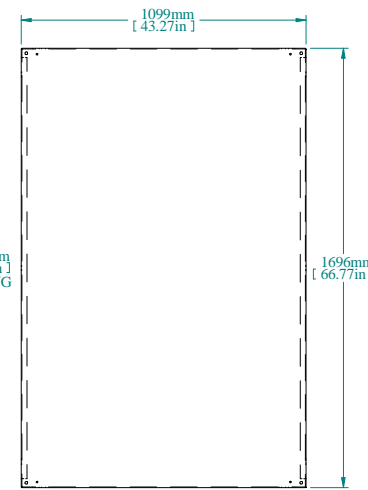
INNER PANEL
