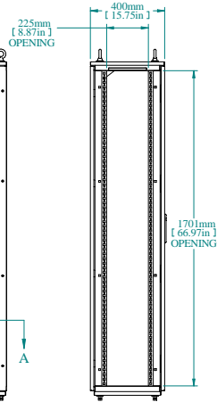
L.S. VIEW
