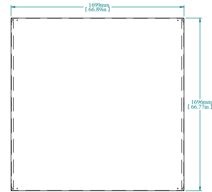
INNER PANEL
