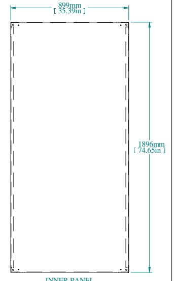
INNER PANEL
