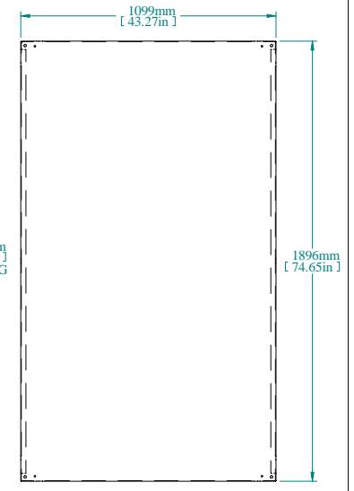
INNER PANEL
