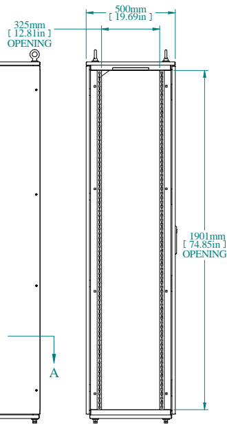
L.S. VIEW
