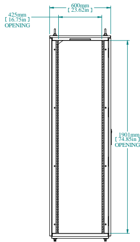
L.S. VIEW
