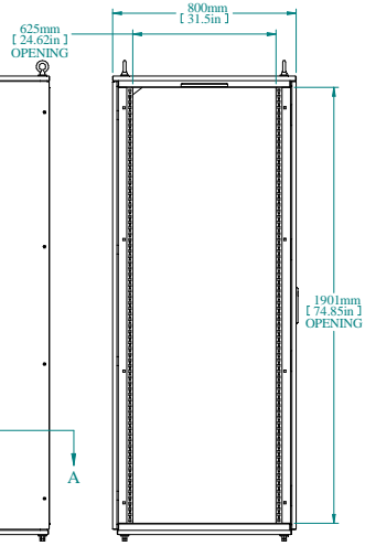
L.S. VIEW
