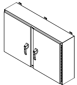
ISOMETRIC VIEW
