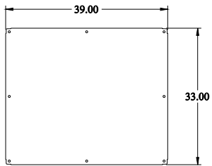
INNER PANEL
