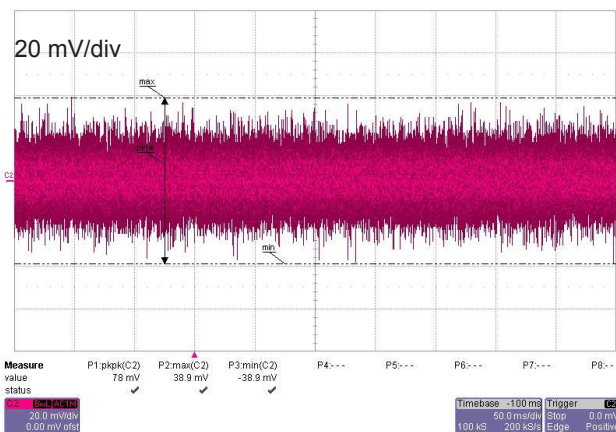
Figure 5: Output noise
