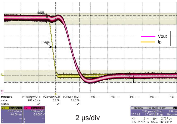
Figure 3: Step response
