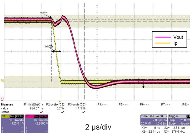
Figure 13: Step response
