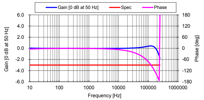
Figure 7: Frequency response
