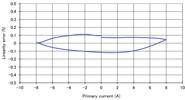
Figure 1: Linearity error
