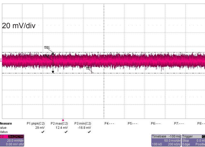
Figure 10: Output noise
