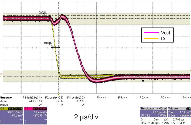
Figure 8: Step response
