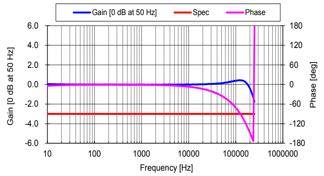
Figure 7: Frequency response
