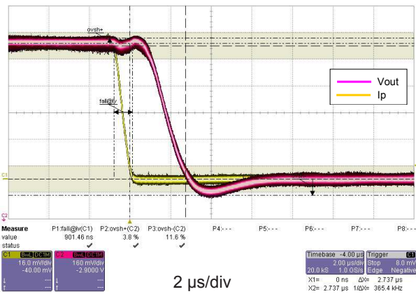
Figure 3: Step response
