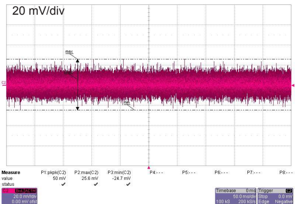
Figure 10: Output noise
