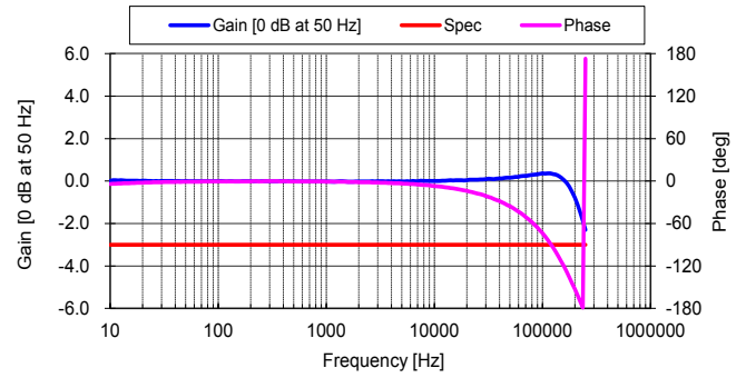
Figure 12: Frequency response
