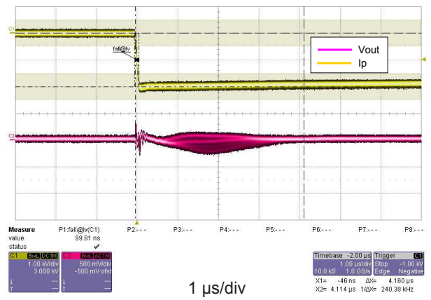
Figure 14: dv/dt
