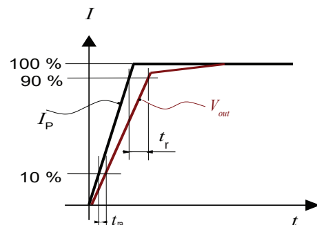
Figure 18: Step response time t_r and reaction time t_{ra}
