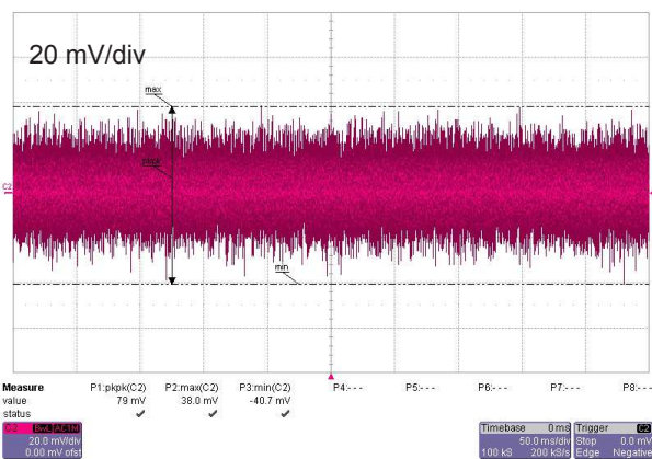
Figure 5: Output noise
