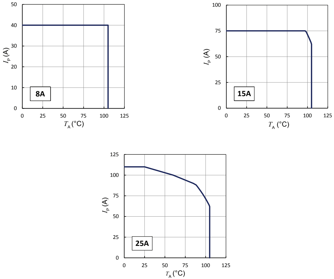
Figure 16: I_p vs T_A for HO series
