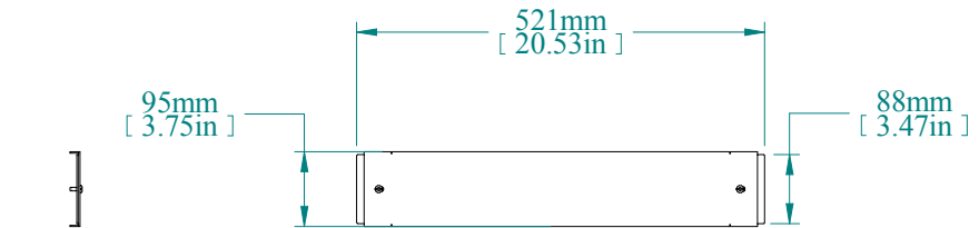
L.S. VIEW
