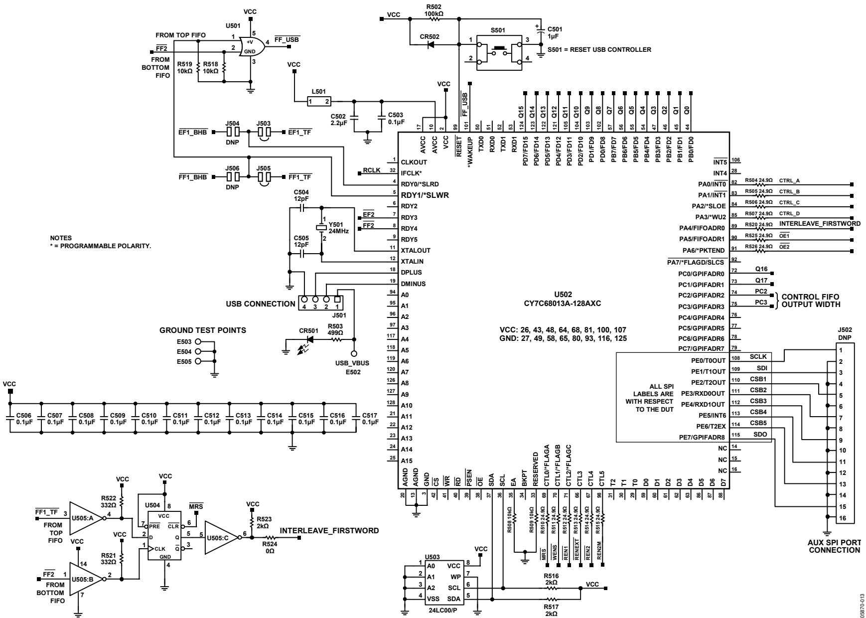
Figure 13. PCB Schematic (Continued)
