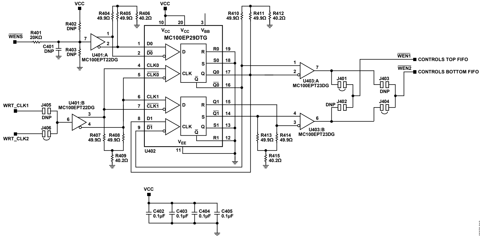
Figure 12. PCB Schematic (Continued)
