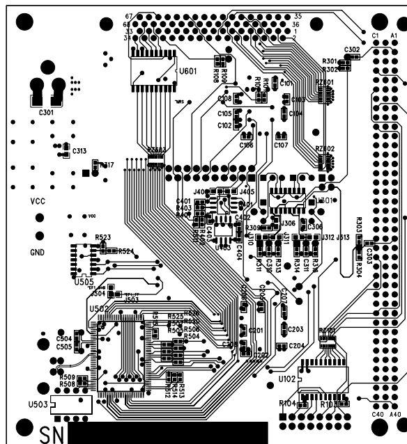
Figure 18. Layer 4—Secondary Side
