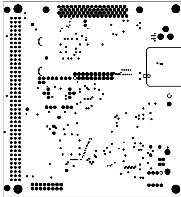
Figure 17. Layer 3—Power Plane
