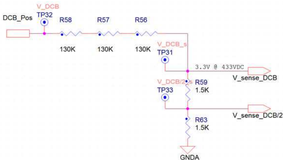
Figure 13. Voltage measurement
