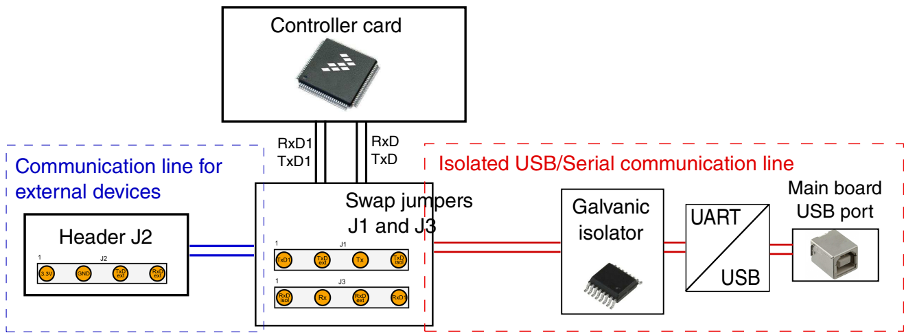
Figure 7. Communication lines
