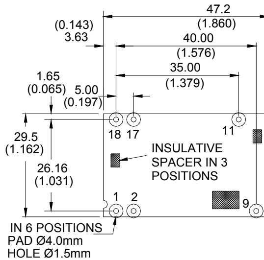
Through-Hole Pad Layout – Component side view
