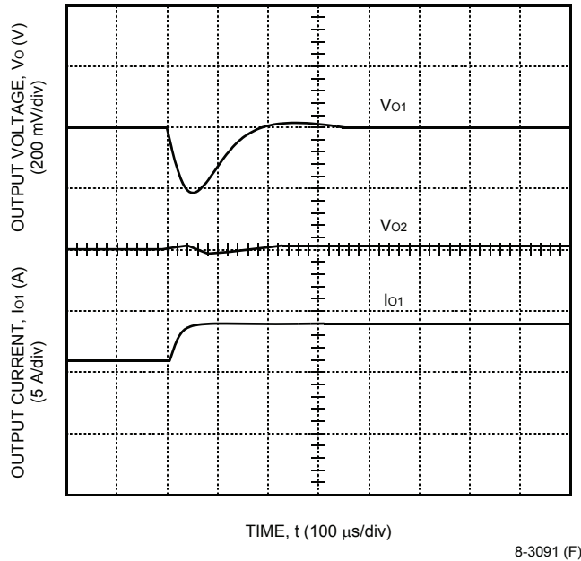
Figure 15. Typical HW050FG1 Transient Response to Step Increase in Load, I_{o1} = 50\% to 75\% of I_{o1, \max} , I_{o2} = 30\% of I_{o2, \max} , at Room Temperature and 48 V Input (Waveform Averaged to Eliminate Ripple Component.)
