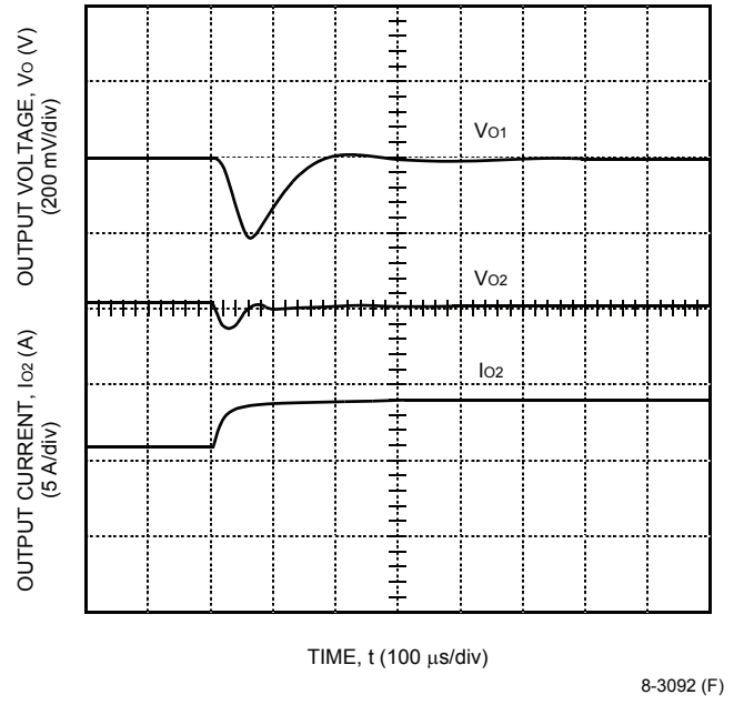
Figure 16. Typical HW050FG1 Transient Response to Step Increase in Load, I_{o2} = 50\% to 75\% of I_{o2, \max} , I_{o1} = 30\% of I_{o1, \max} , at Room Temperature and 48 V Input (Waveform Averaged to Eliminate Ripple Component.)
