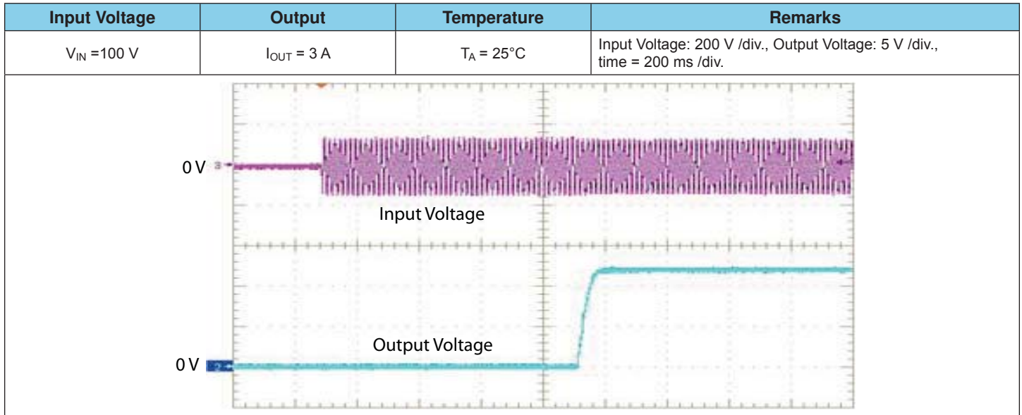
Figure 9. Output Voltage Rising
