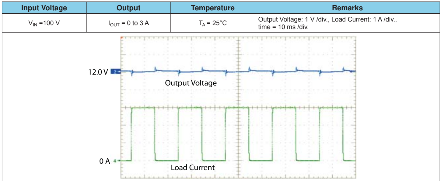
Figure 20. Dynamic Load
