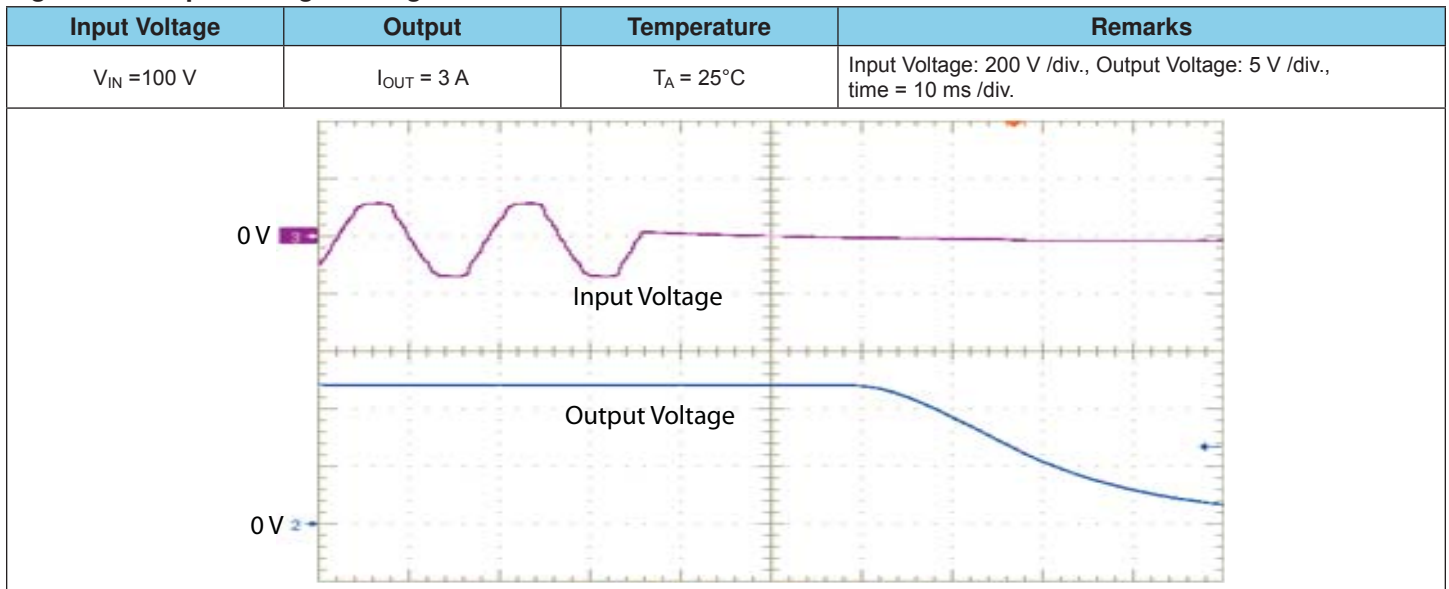
Figure 10. Output Voltage Falling
