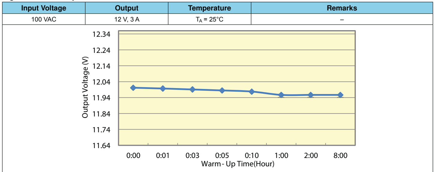
Figure 11. Warm-Up Drift
