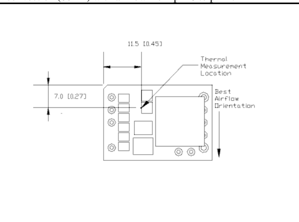
i6A24014A033V thermal measurement location – top view
