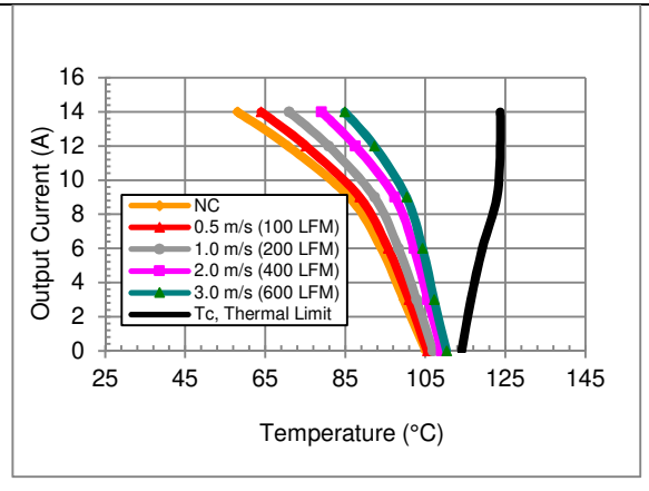
Vo=12V, Vin=24V preliminary maximum output current vs. ambient temperature at nominal input voltage for natural convection (60lfm) with airflow from pin 8 to pin 4.
