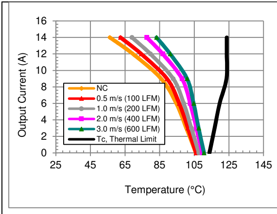
Vo=18V, Vin=24V preliminary maximum output current vs. ambient temperature at nominal input voltage for natural convection (60lfm) with airflow from pin 8 to pin 4.
