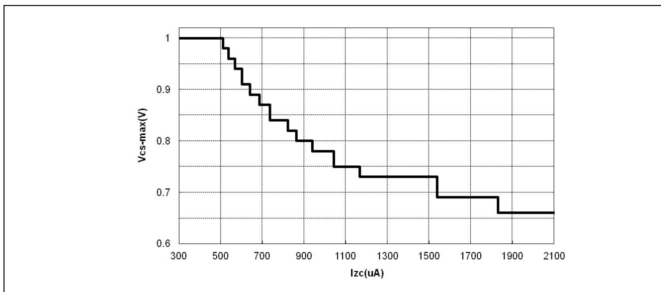
Figure 8 V_{CS-max} versus I_{ZC}
