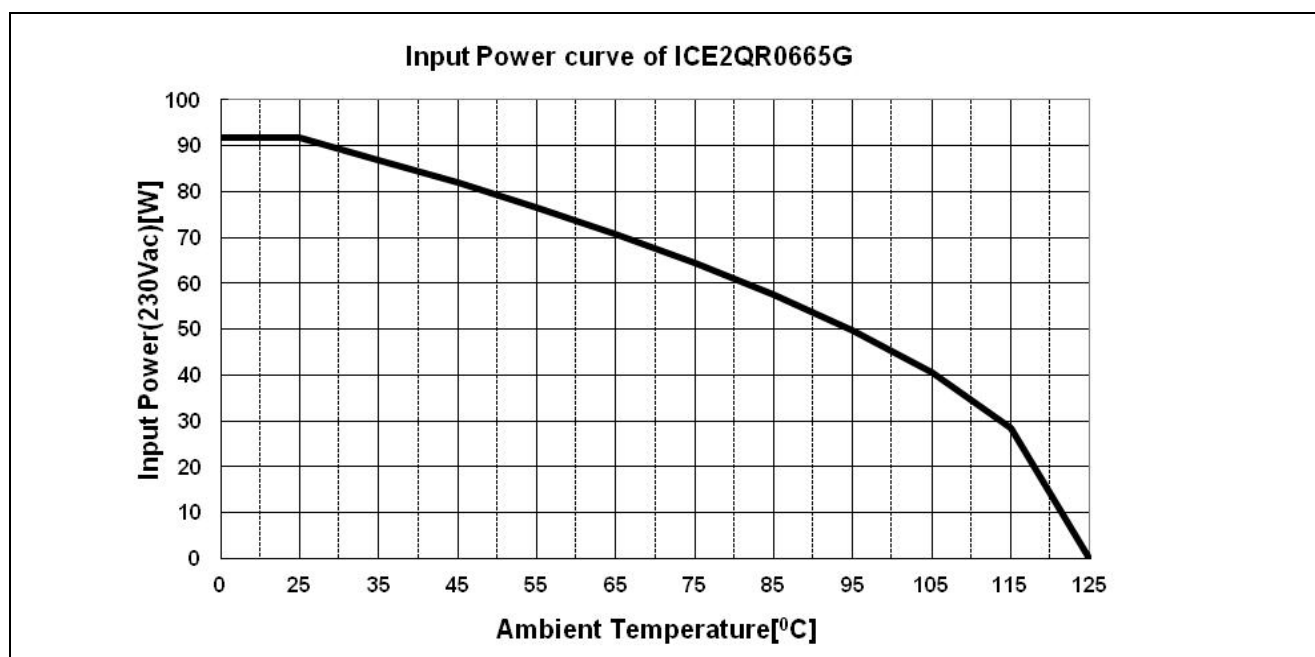
Figure 14 Input Power curve V_{in}=230\text{Vac} ; P_{in}=f(T_a)
