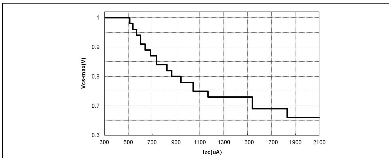
Figure 8 V_{CS-max} versus I_{ZC}
