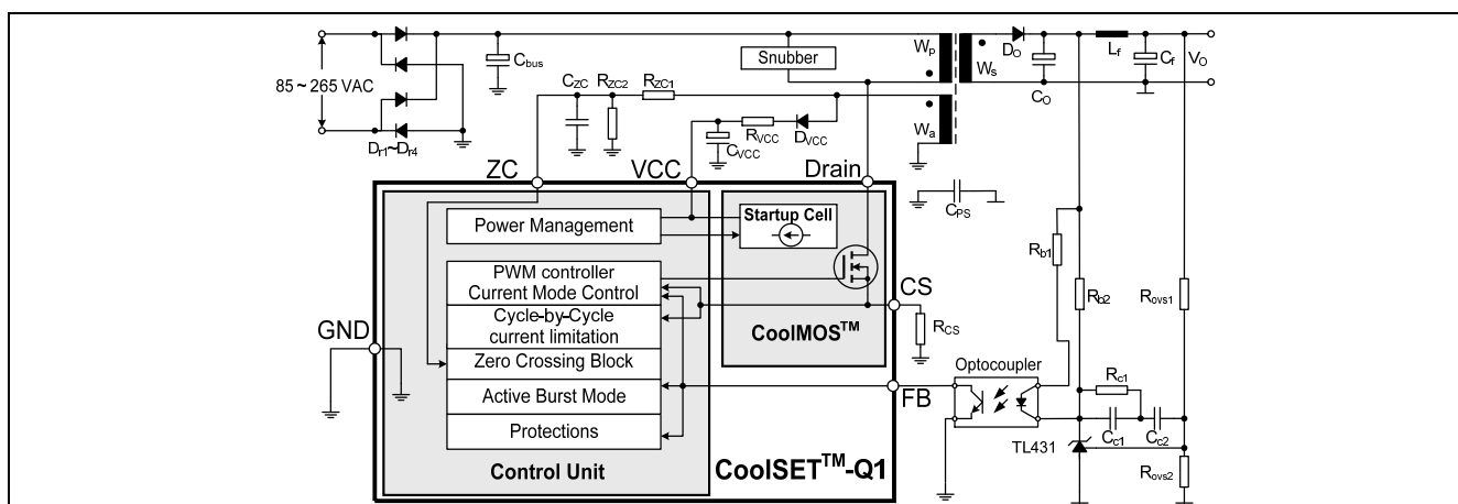
Figure 1 Typical Application
