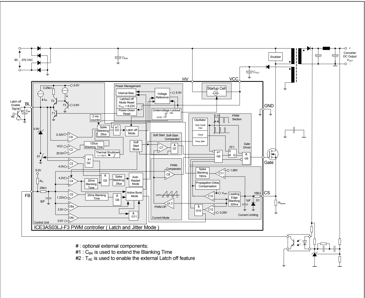
Figure 2 Representative Blockdiagram
