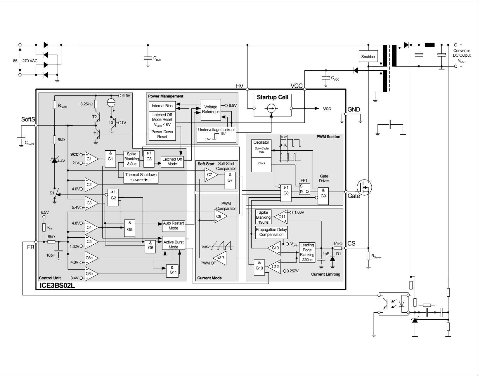
Figure 2 Representative Blockdiagram
