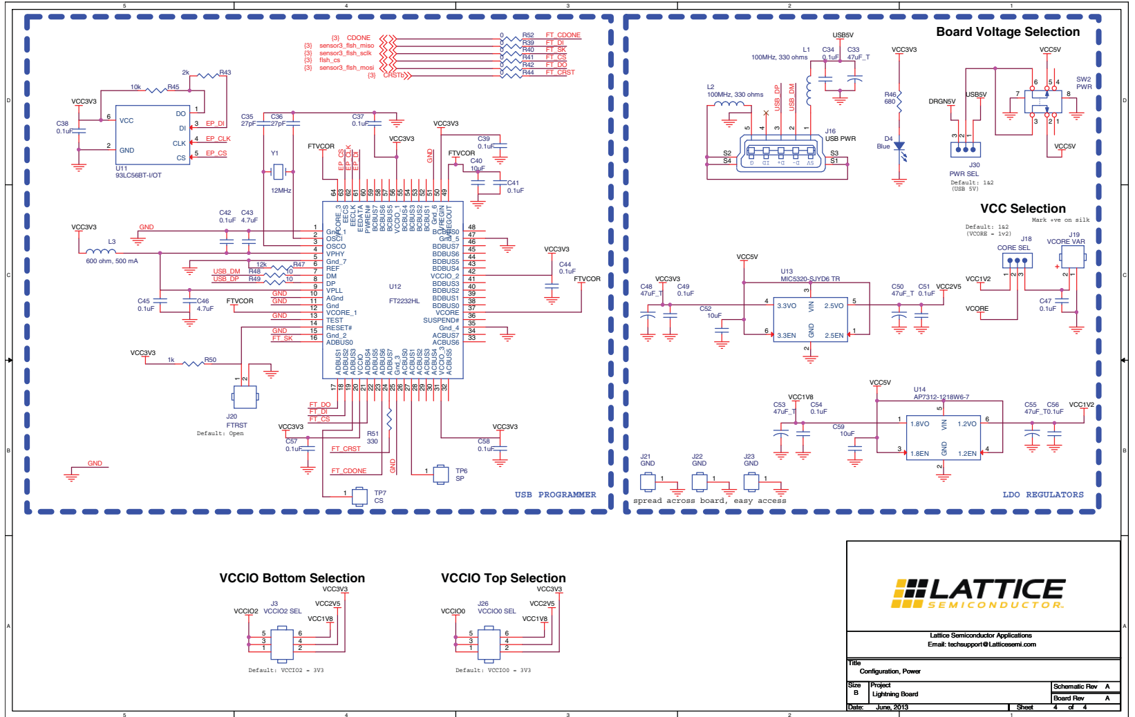
Figure 15. Configuration and Power
