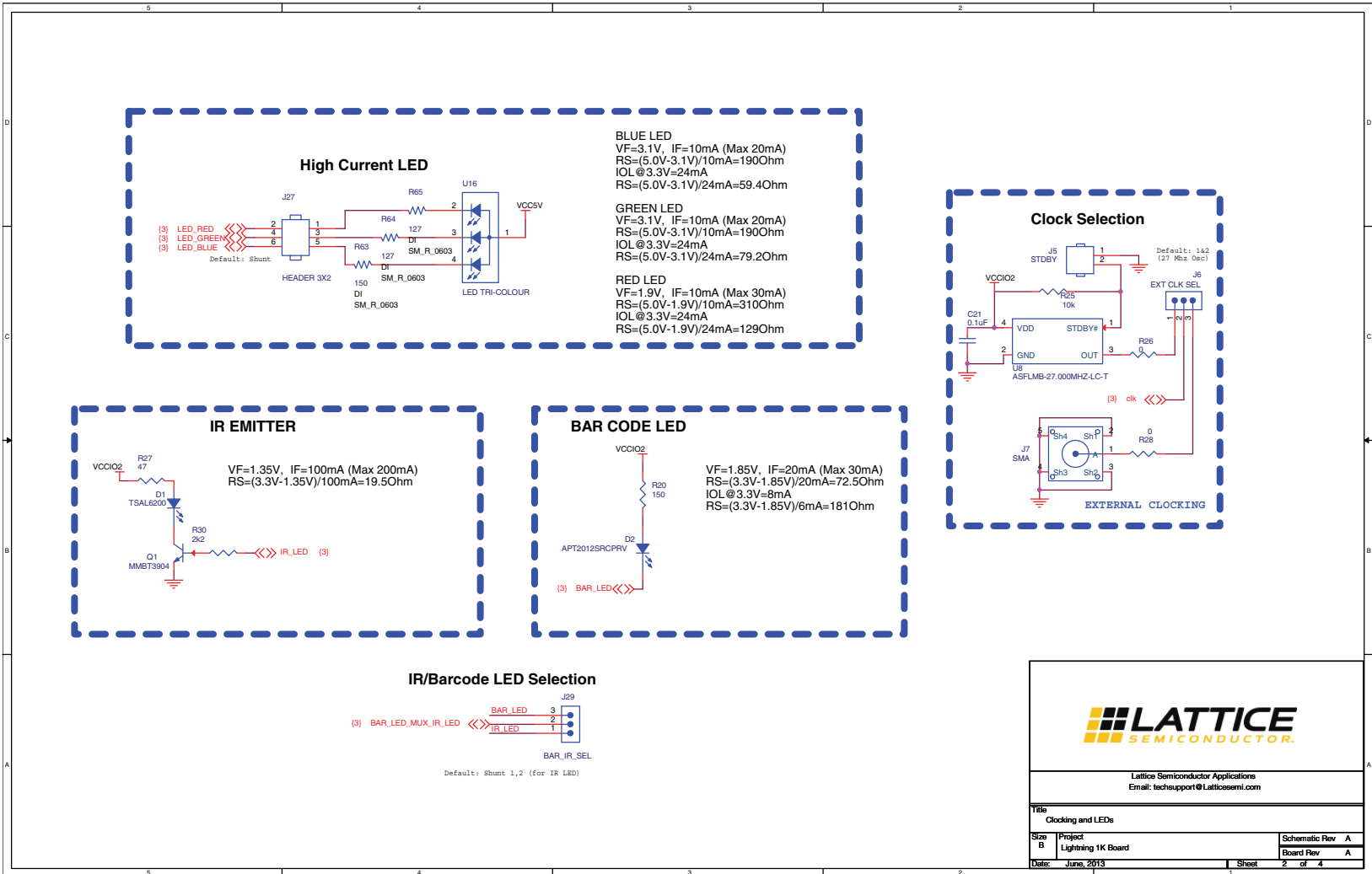
Figure 13. Clocking and LEDs
