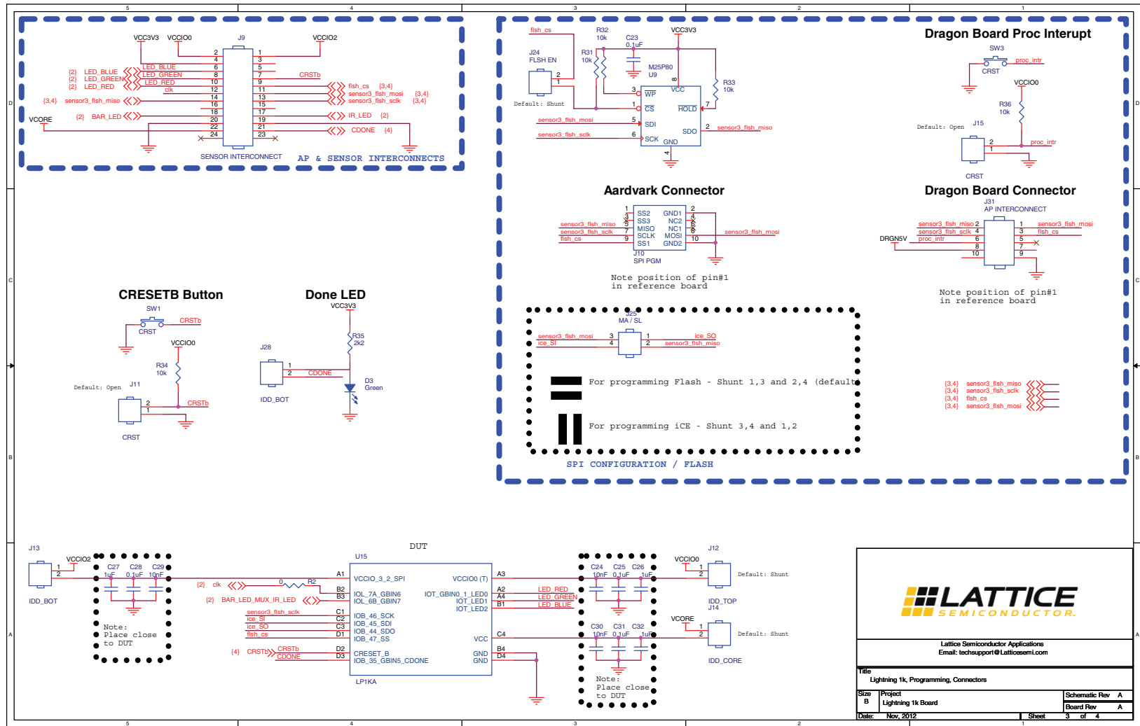
Figure 14. Programming and Connectors
