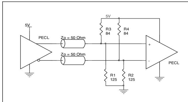
FIGURE 6B. 5V LVPECL OUTPUT TERMINATION EXAMPLE
