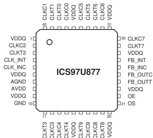
40-Pin MLF
