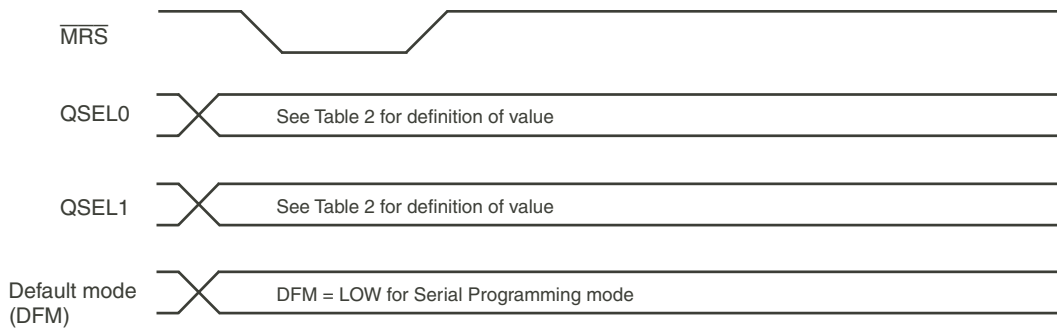
Figure 3. Reference Signals
