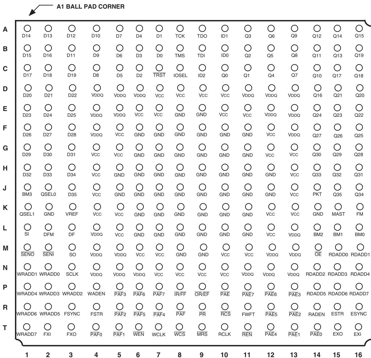
PBGA (BB256-1, order code: BB) TOP VIEW
