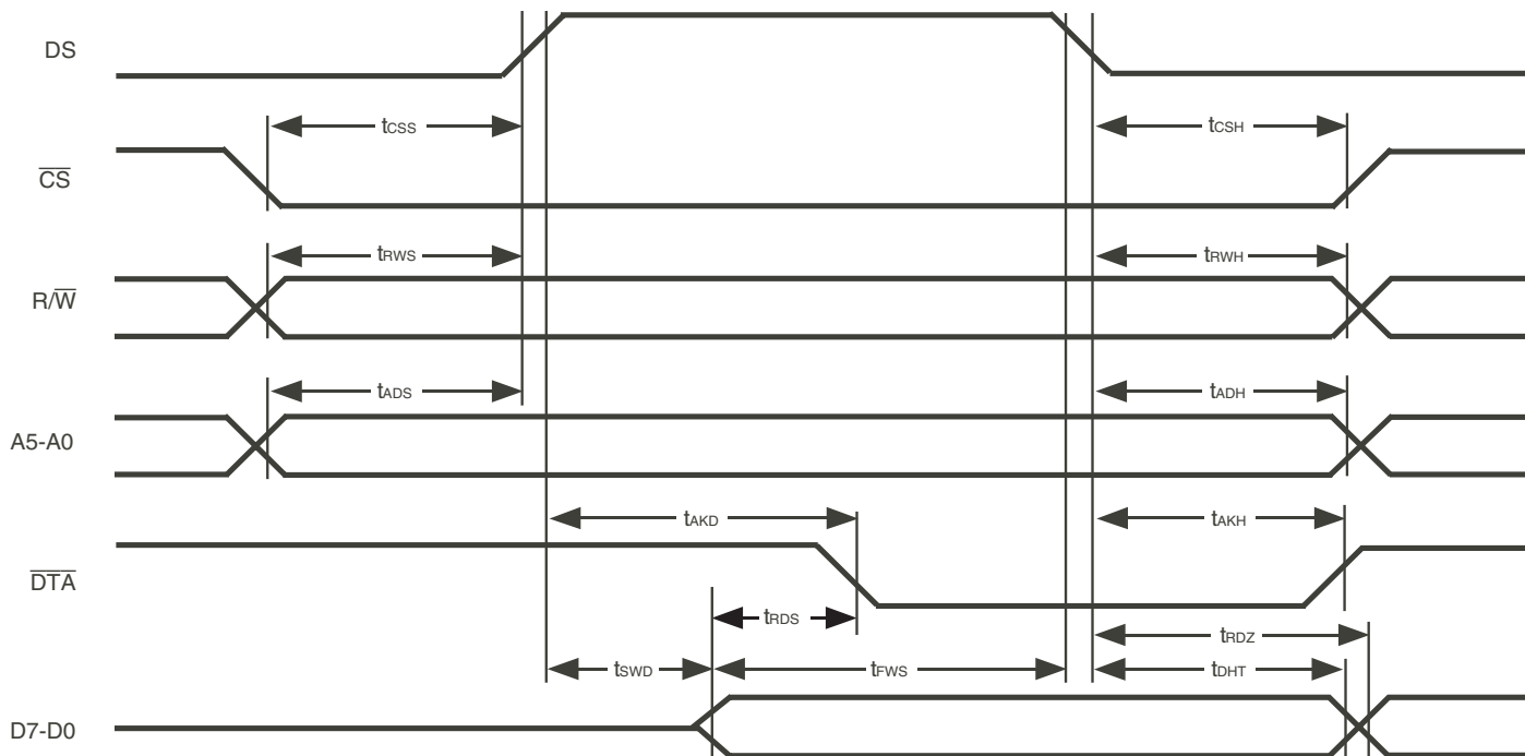
Figure 10. Processor Bus
