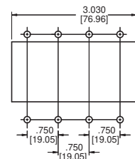
Panel Mounting Detail Tolerance \pm .005 [.13] unless noted.
