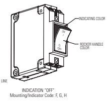
INDICATION "OFF" Mounting/Indicator Code: F, G, H
