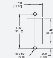
Panel Mounting Detail Mounting Detail Tolerance: \pm .005 [.13] unless noted
