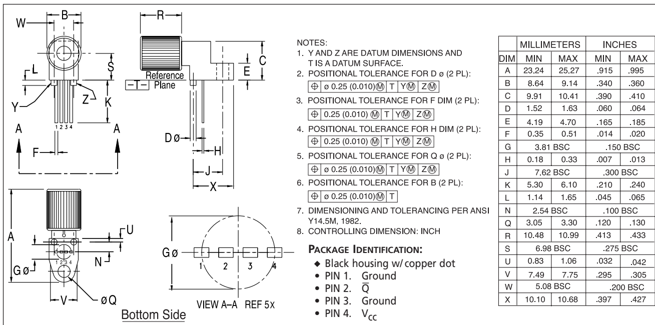
FIGURE 4. Case outline.
