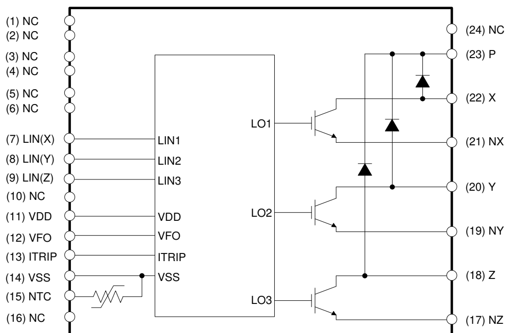
Figure 2 Internal schematic
