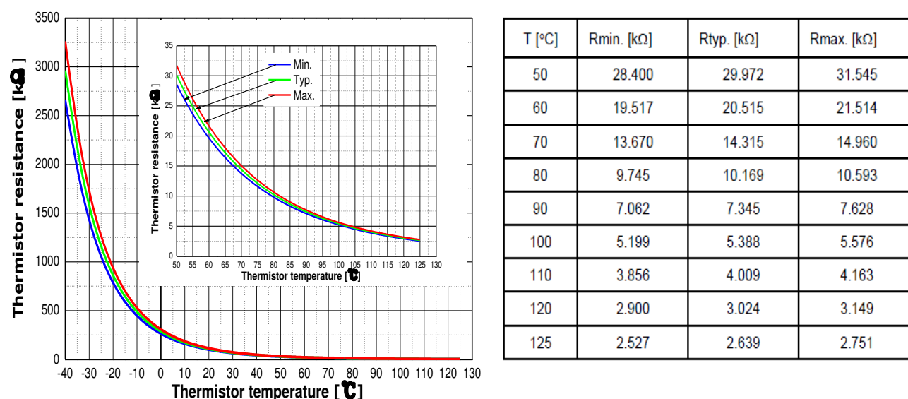
Figure 7 Thermistor resistance – temperature curve and table (For more information, please refer to the application note 'AN CIPOS™-Mini 1 Technical description')
