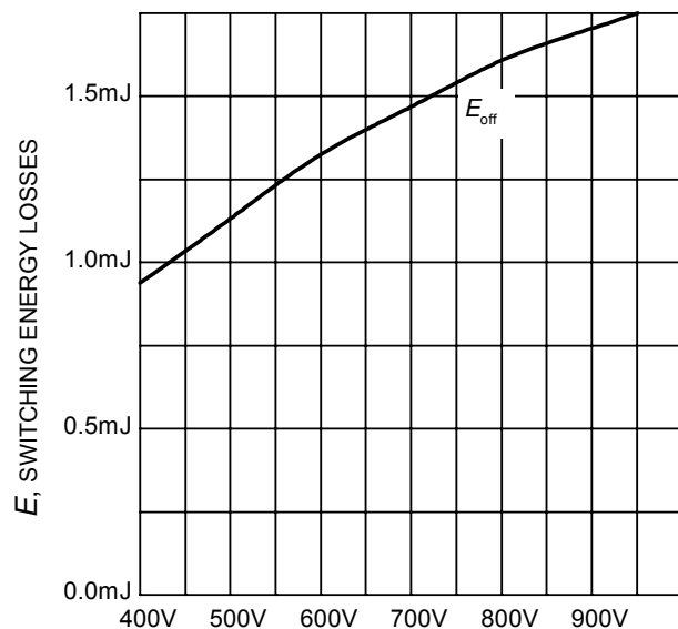
Figure 16. Typical turn-off energy as a function of collector emitter voltage (inductive load, T_J=175^\circ\text{C} , V_{GE}=0/15\text{V} , I_C=15\text{A} , R_G=14.8\Omega , Dynamic test circuit in Figure E)
