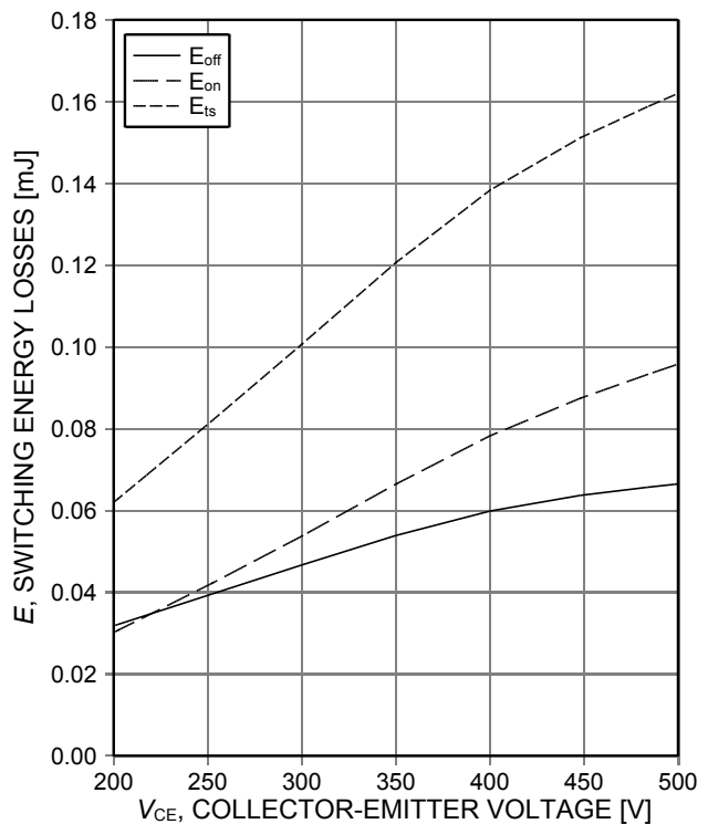
Figure 16. Typical switching energy losses as a function of collector emitter voltage (inductive load, T_{vj}=175^\circ\text{C} , V_{GE}=0/15\text{V} , I_c=2,5\text{A} , R_{Gon}=68\Omega , R_{Goff}=68\Omega , dynamic test circuit in Figure E)
