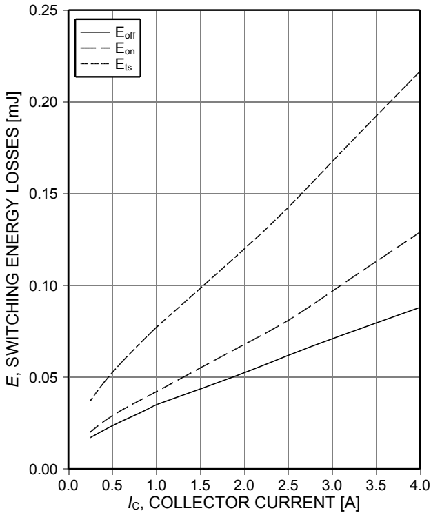
Figure 13. Typical switching energy losses as a function of collector current (inductive load, T_{vj}=175^\circ\text{C} , V_{CE}=400\text{V} , V_{GE}=0/15\text{V} , R_{Gon}=68\Omega , R_{Goff}=68\Omega , dynamic test circuit in Figure E)
