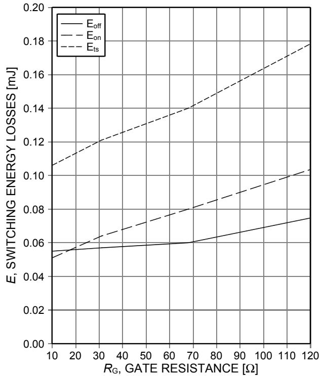
Figure 14. Typical switching energy losses as a function of gate resistance (inductive load, T_{vj}=175^\circ\text{C} , V_{CE}=400\text{V} , V_{GE}=0/15\text{V} , I_c=2,5\text{A} , dynamic test circuit in Figure E)
