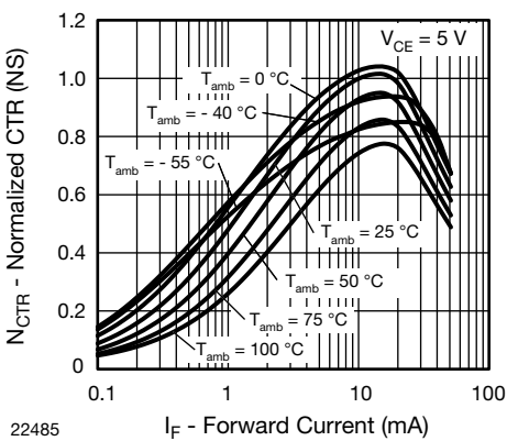
Fig. 7 - Normalized CTR (non-saturated) vs. Forward Current
