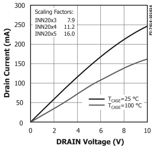
Figure 20. Output Characteristic.
