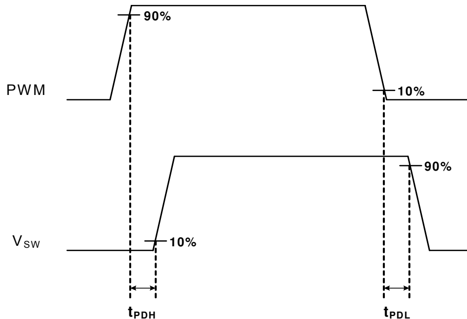
Figure 10 Timing Diagram
