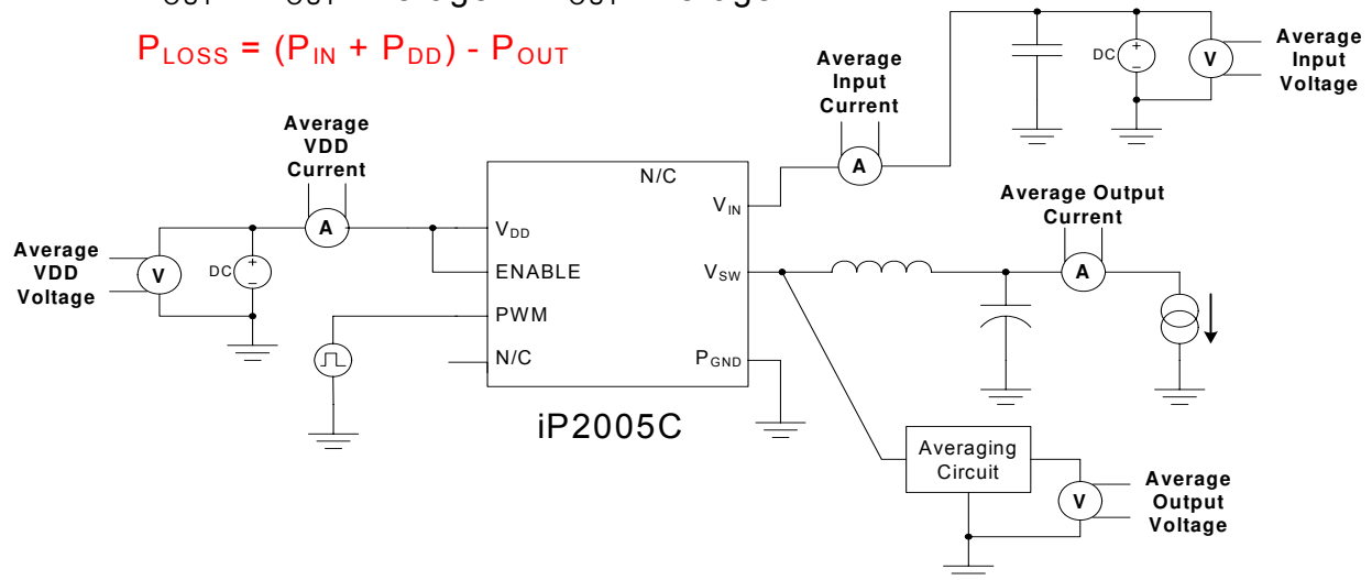
Figure 9 Power Loss Test Circuit
