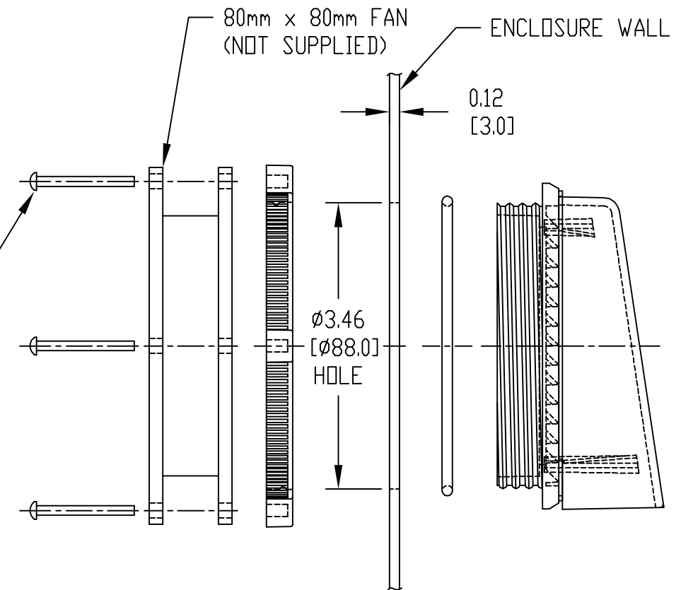
TYPICAL INSTALLATION
